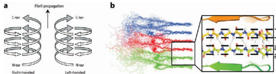
Figure 7. (a) Models for right-handed and left-handed \beta -solenoids. (b) Backbone side view of three consecutive molecules (bundle of the 20 lowest energy structures) and stick representation of the intermolecular interface of two consecutive HET-s(218–289) molecules in the fibril. The short intermolecular H^N-H^{\alpha} distances are displayed as dashed lines. The distances d_1 and d_2 (approximately corresponding to H^N-H^{\alpha} distances between two consecutive \beta -sheet layers) are about 2.7 and 7.5 Å, respectively.
